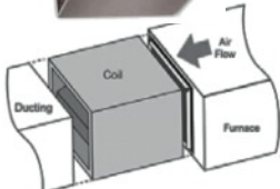
Fig 5B-1. Horizontal Left Application
